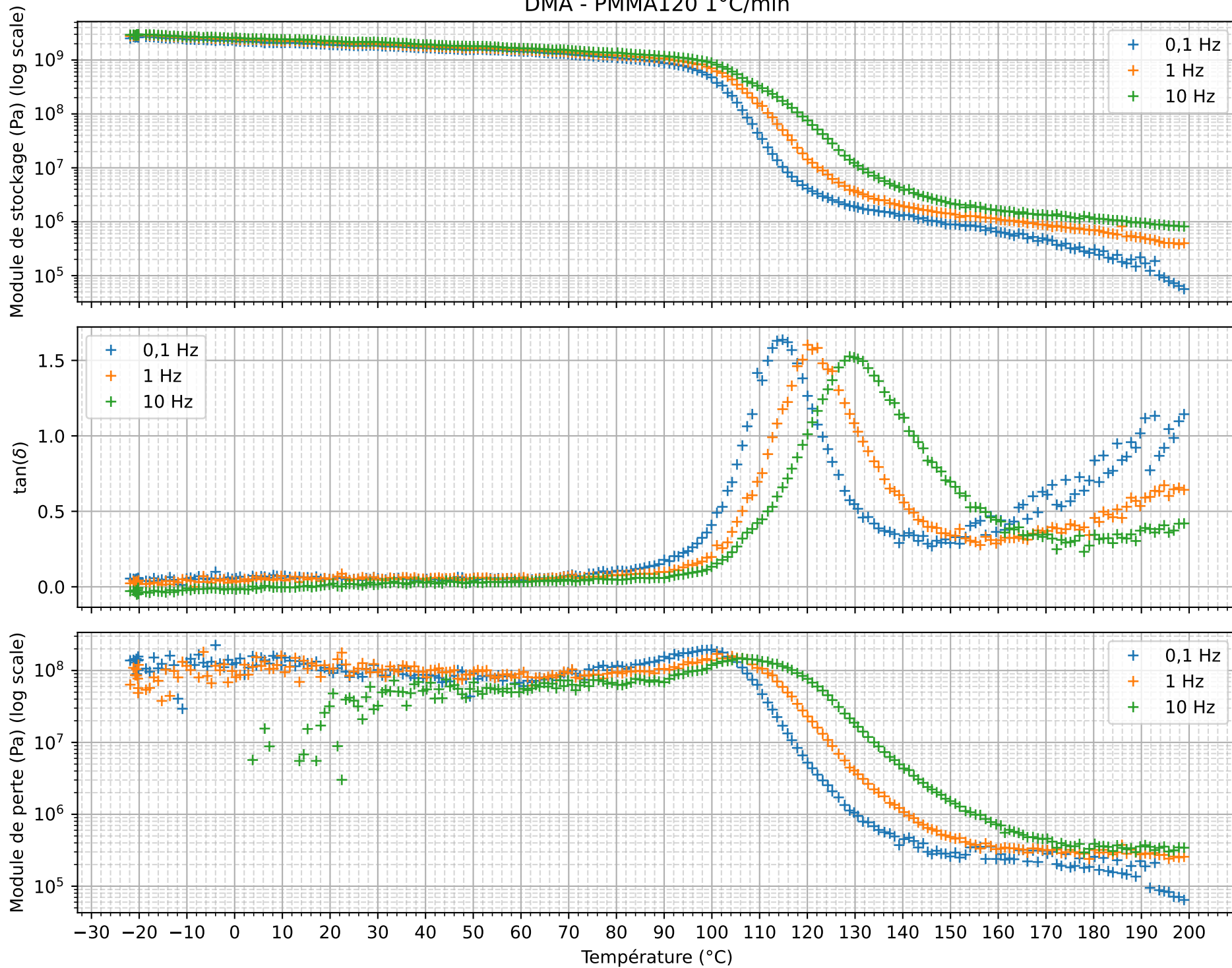
DMA - PMMA120 1°C/min
